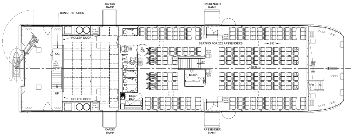
MAIN DECK
