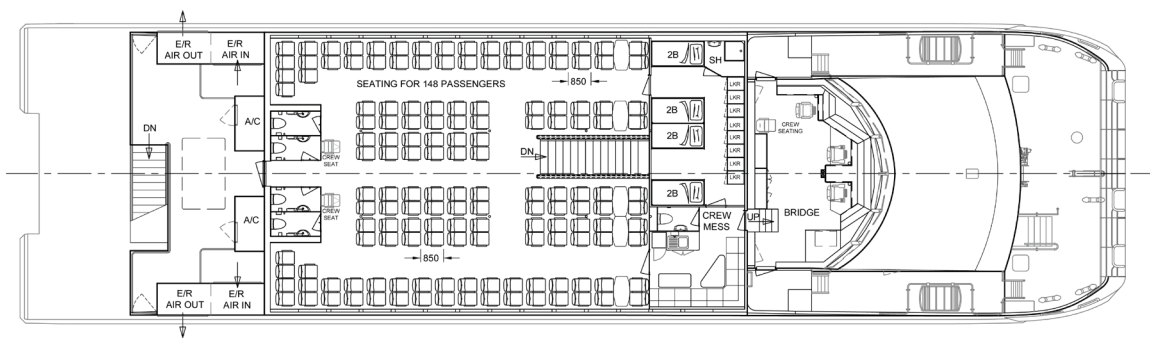
UPPER DECK
